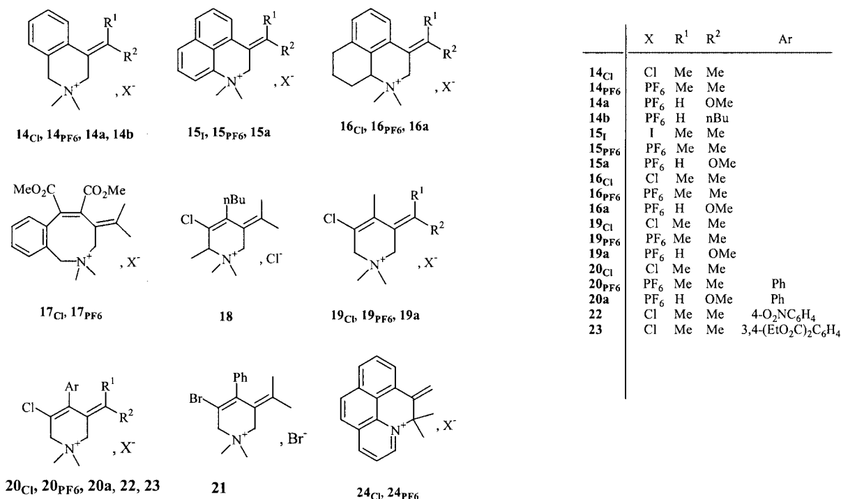
Figure 2. Structures of the various cationic N-heterocyclic compounds obtained
