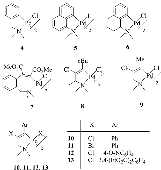
Figure 1. Structures of the various cyclopalladated starting complexes
